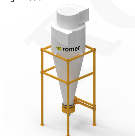
Cyclone separators
